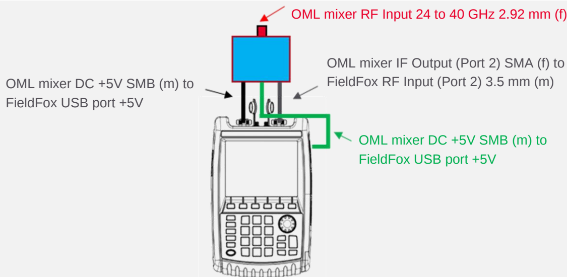
Figure 1. OML external mixer diagram 1
