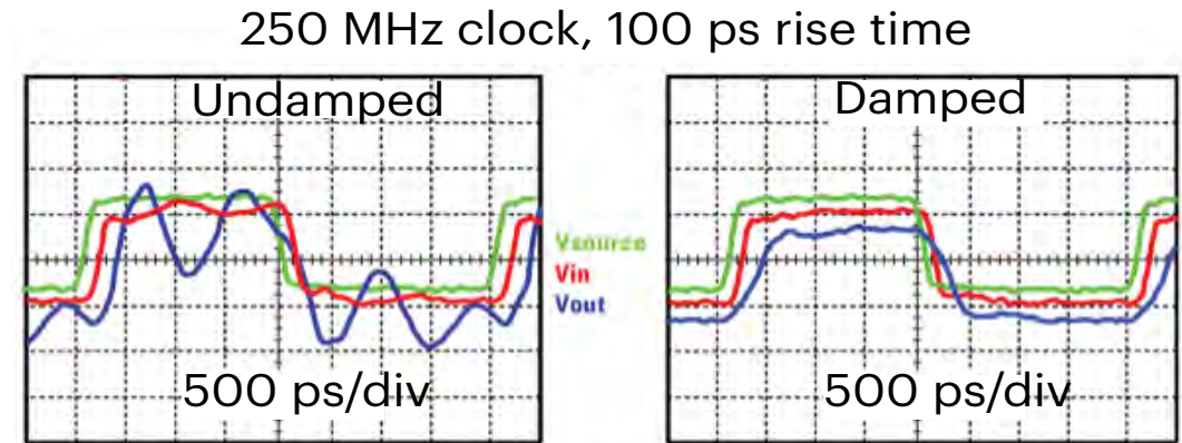
Figure 5. Adding a resistor to a probe tip can overcome resonance from long probe connections, reduce ringing and overshoot. However, it will not prevent bandwidth limiting caused by the added leads.
